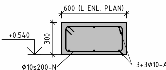
S08 1 : 20 SULA UNDER TRAPPA
