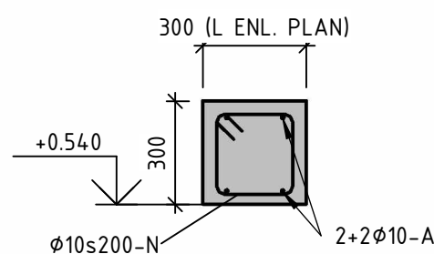
S09 1 : 20 SULA UNDER VILPLAN TRAPPA
